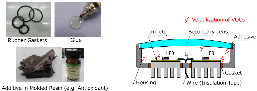
Figure 2. Examples of Surrounding Materials that may Release VOCs
