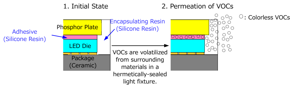
Figure 4. VOC Permeation
