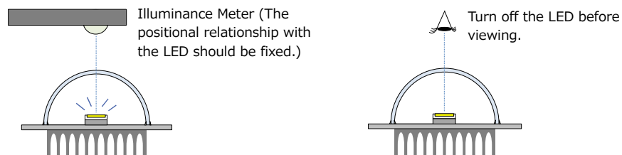
Figure 11. How to Check Luminous Intensity and Discoloration
