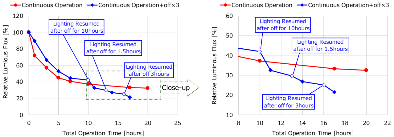
Figure 14. Comparison of Continuous Operation and On/Off Operation
