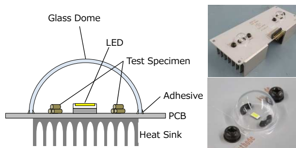
Figure 9. Example of Test Apparatus for VOC Discoloration Test
