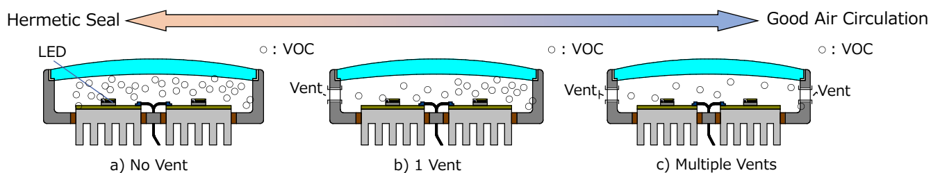
Figure 7. Example of Preventive Measure (Ventilation)
