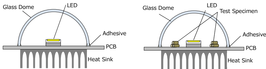
Figure 10. Test Method Examples (Left: Reference; Right: Apparatus with Test Specimen)
