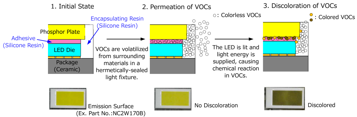
Figure 6. VOC Discoloration
