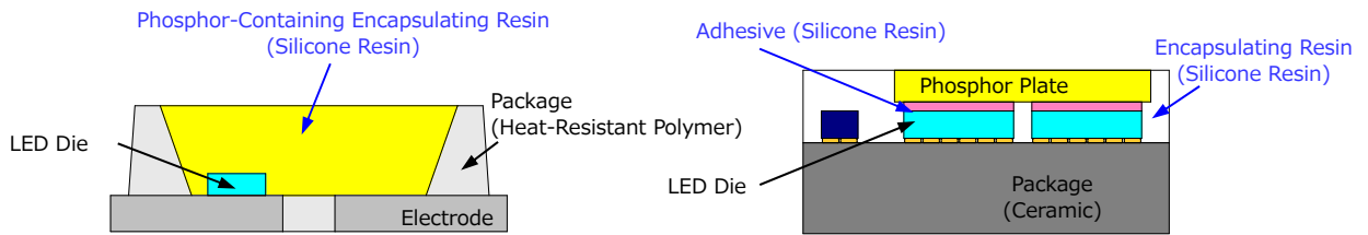
Figure 3. Examples of Silicone Resins Used in LED
