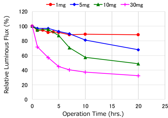
Figure 13. Diphenylamine Amount vs. Decrease in the Luminous Flux in a Hermetically-Sealed Environment
