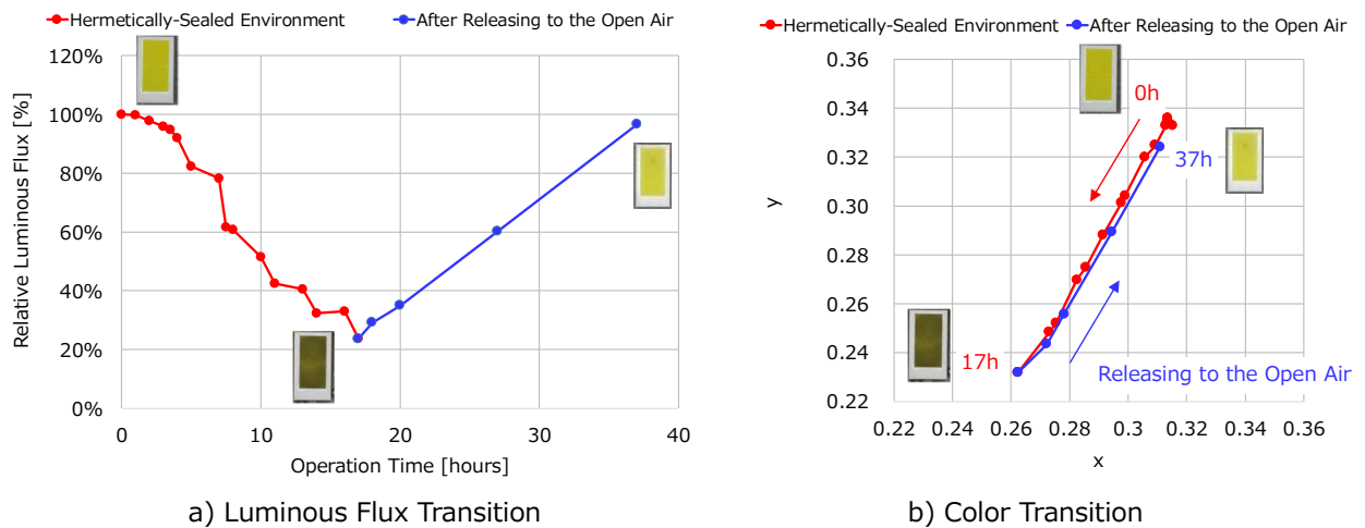
Figure 12. Discoloration of VOCs and Reduction in the Discoloration (Verification by Accelerated Test Under High VOC Concentration)
