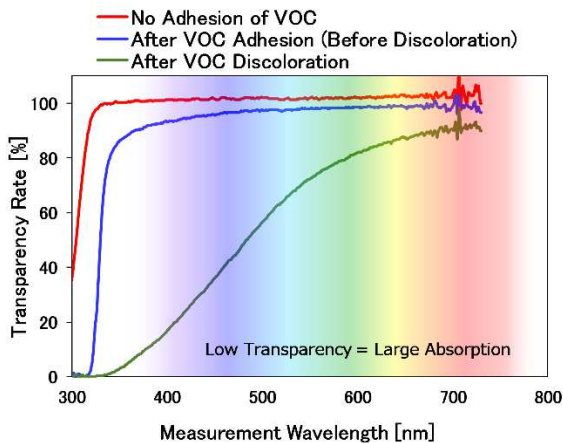
Figure 5. Transparency Change due to VOC Adhesion and Discoloration
